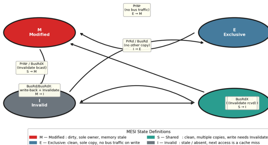
Figure 4: Complete MESI Cache Coherence State Transition Diagram PrRd/PrWr = Processor Read/Write. BusRd/BusRdX = Bus Read / Read-Exclusive (with Invalidate)
